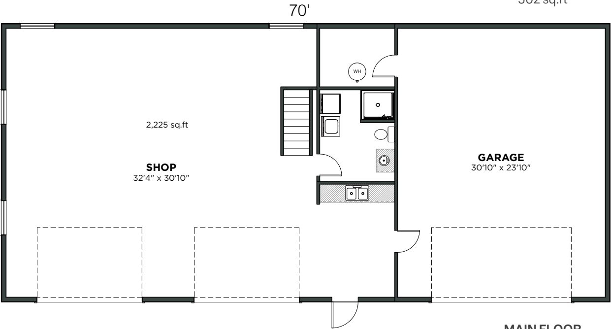
MAIN FLOOR 2,225 sq.ft
