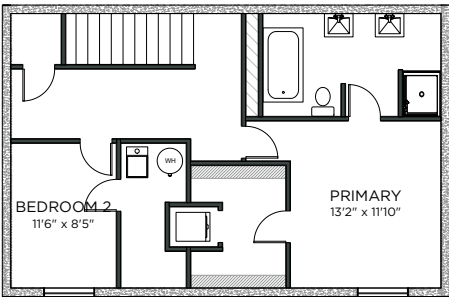
LOWER FLOOR 730.24 sq.ft
