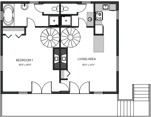
UPPER FLOOR 990 sq.ft
